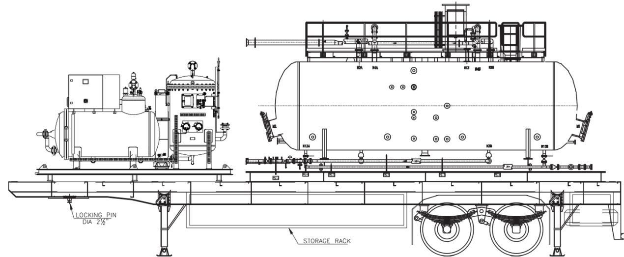
DESALTER & DEOILER
