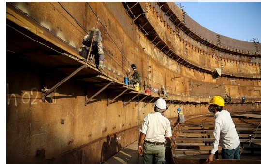
Cooperation and supply in production of 12,000 MT of A516Gr.70+N sheets for Assaluyeh Green Reservoir Project
